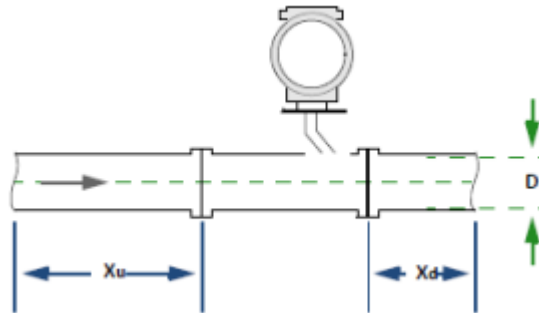
Image 4. Installation of In-line Meters (representative)
