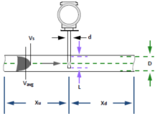
Image 3. Installation of Insertion Meters (representative)
